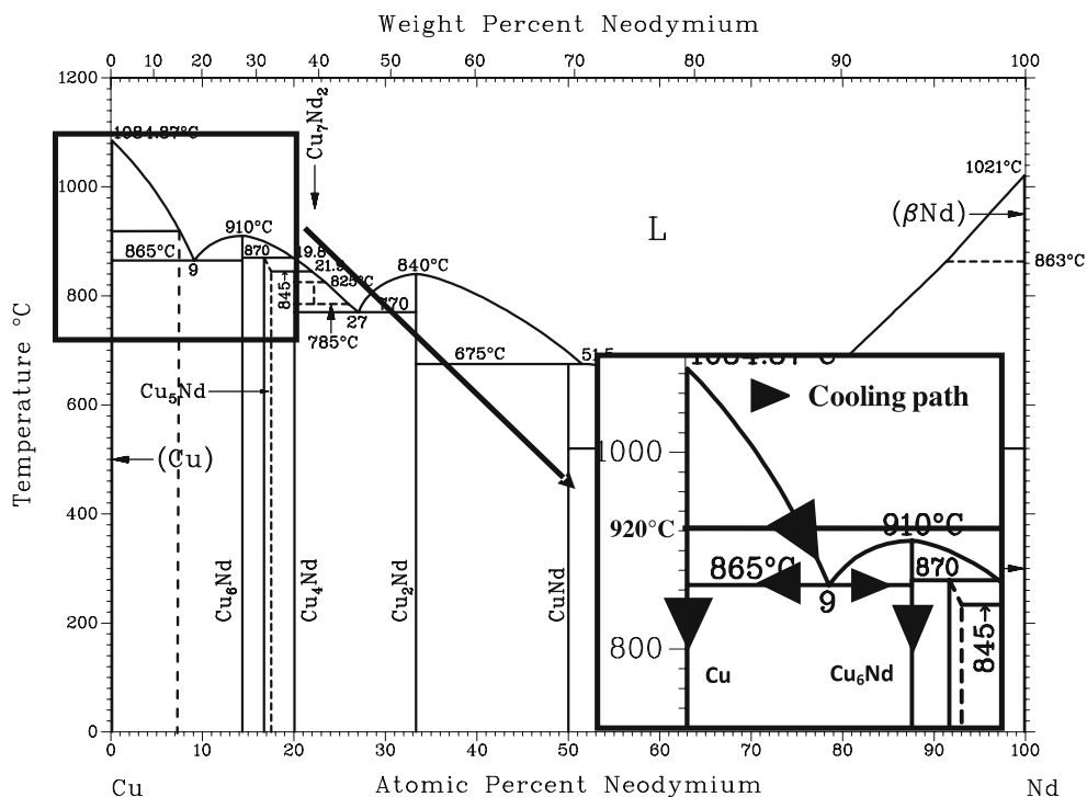
Fig. 10 Cu–Nd phase diagram [15]. Cooling path of the Cu/Cu 6 Nd eutectic
