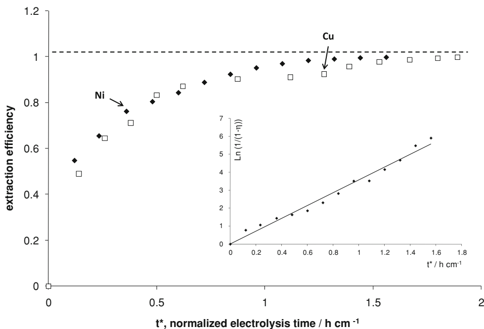
Fig. 6 Variation of the extraction efficiency of Nd at 840 °C on copper and nickel electrodes versus t^* , the normalized electrolysis time. Inset: Linear relationship between \ln(1/(1-\eta)) and t^* for Nd extraction on nickel at 840 °C
