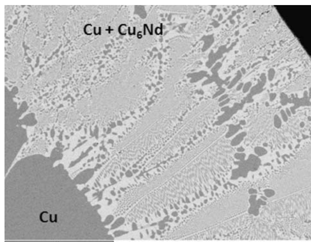
Fig. 9 SEM micrograph of a copper electrode used for the extraction electrolysis at 920 °C
